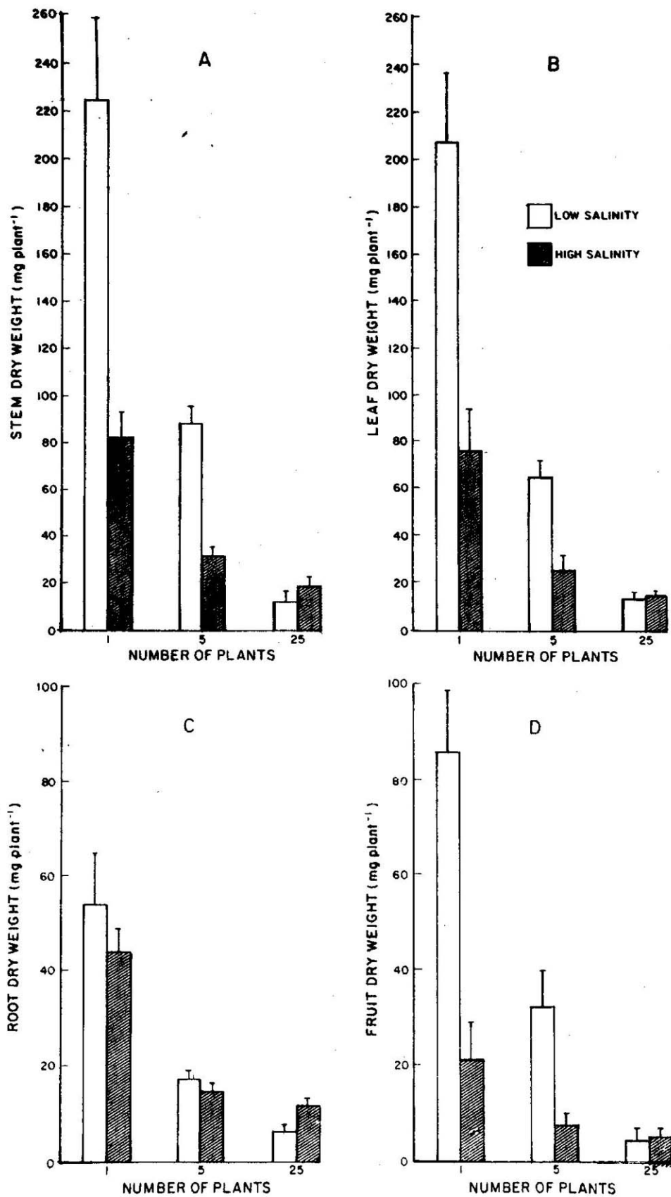
Fig. 1. Effect of salinity and density on the growth and reproduction of Atriplex triangularis plants grown under saline conditions.
